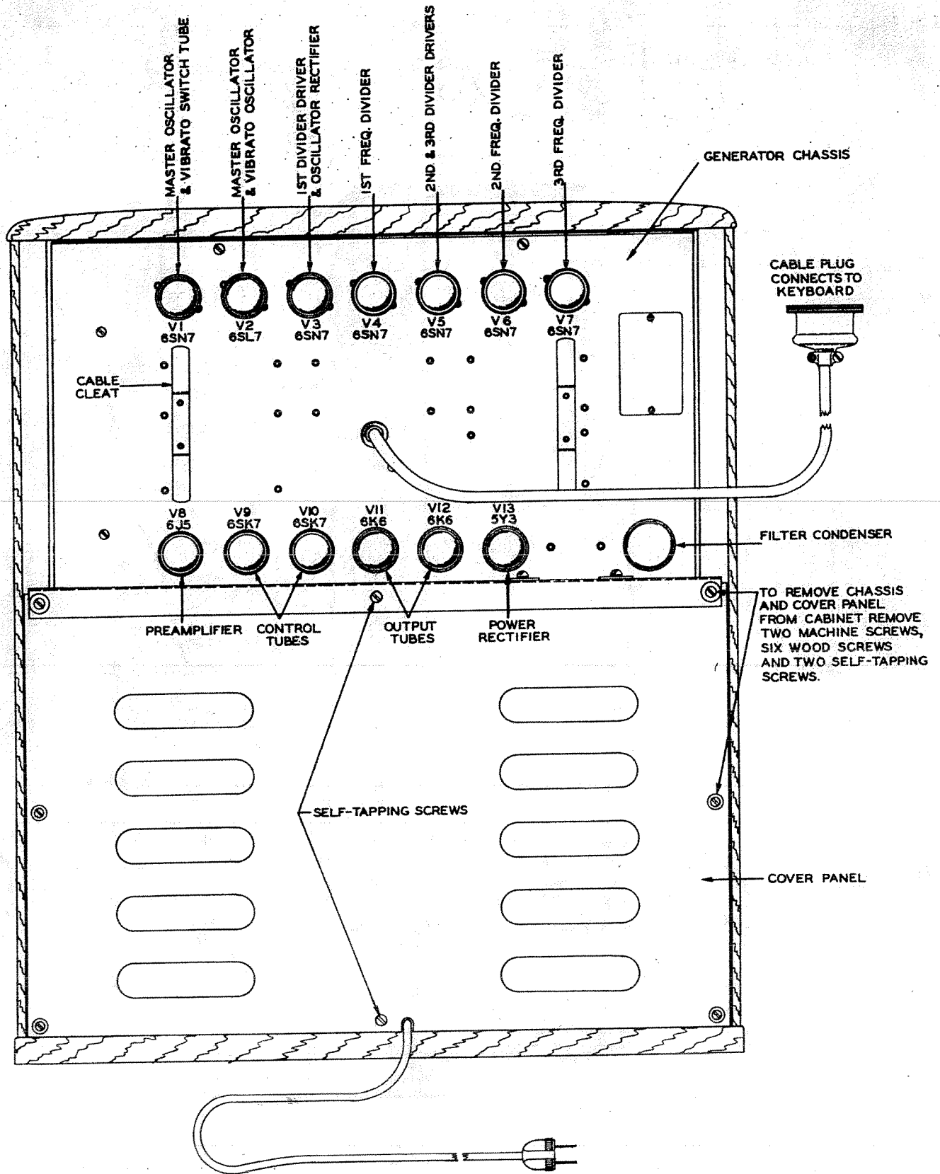
REAR VIEW OF TONE CABINET SOLOVOX MODEL L
